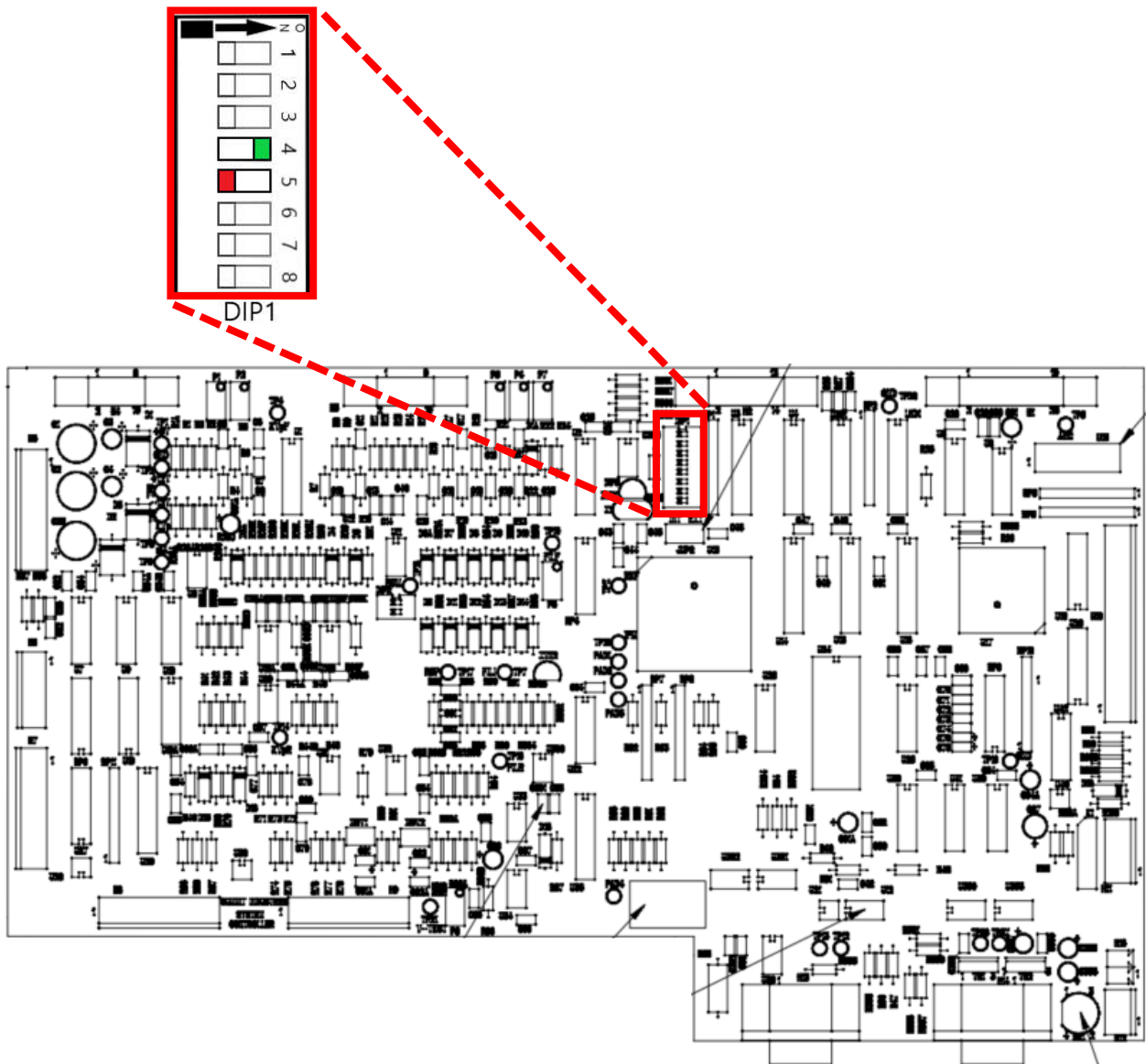
System Controller Board
