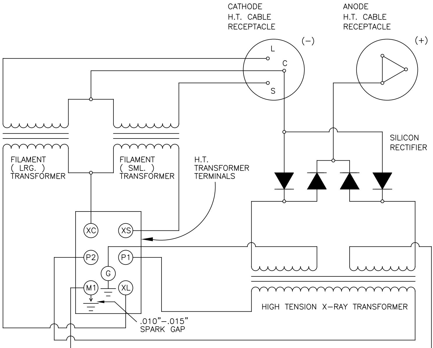
HIGH TENSION TRANSFORMER DIAGRAM A700
